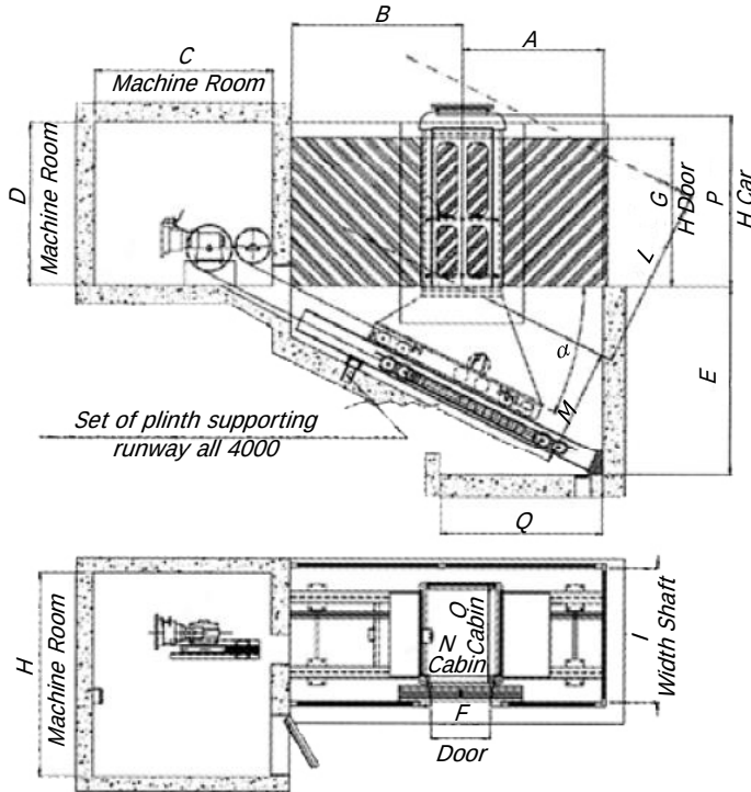
Inclined Lift in opened shaft panoramic car
