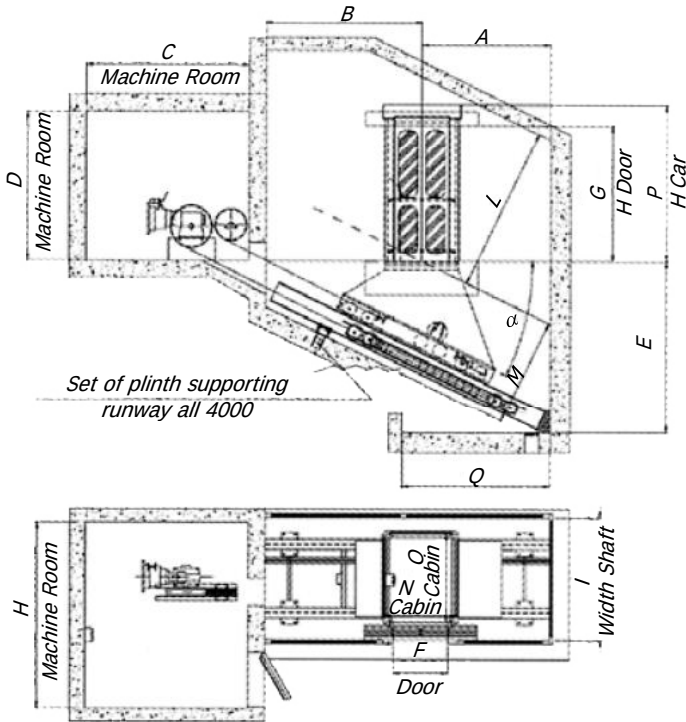
Inclined Lift in closed shaft
